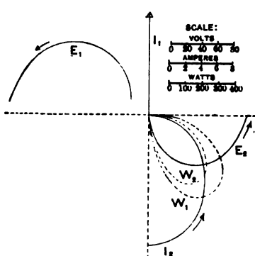
FIG. 10.—Constant Current, Step Down, Arm at 180°
